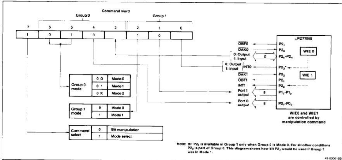
Figure 11. Mode 1 Output
