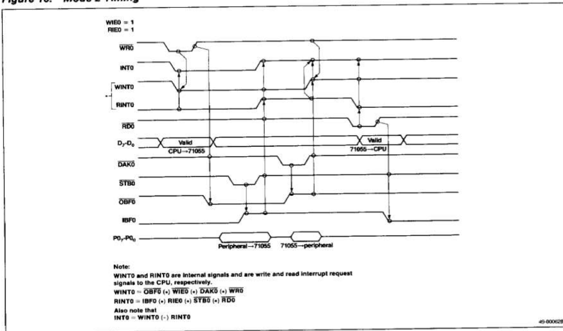
Figure 16. Mode 2 Timing
