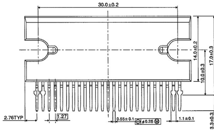
OUTLINE DRAWING HZIP25-P-1.27C
