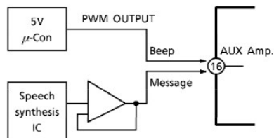
(Fig.7) The application of AUX. amplifier
