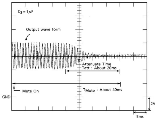
(Fig.4) Output wave form at Muting Condition
