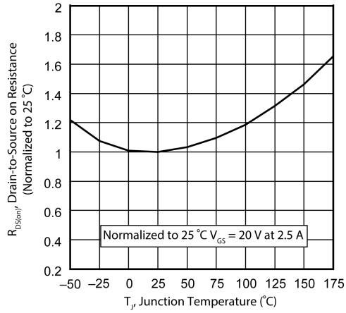
Figure 5 • RDS(on) vs. Junction Temperature
