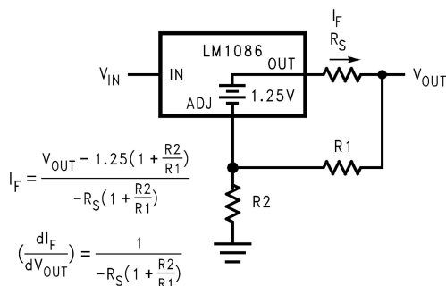
Figure 21. Battery Charger
