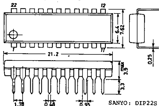
Package Dimensions 3059-D22SIC (unit: mm) [LC7364J]
