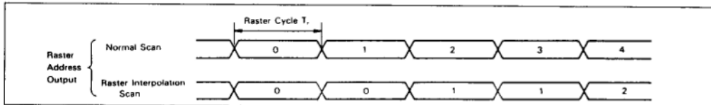
Figure 15 Raster Address Output and Raster Interpolation
