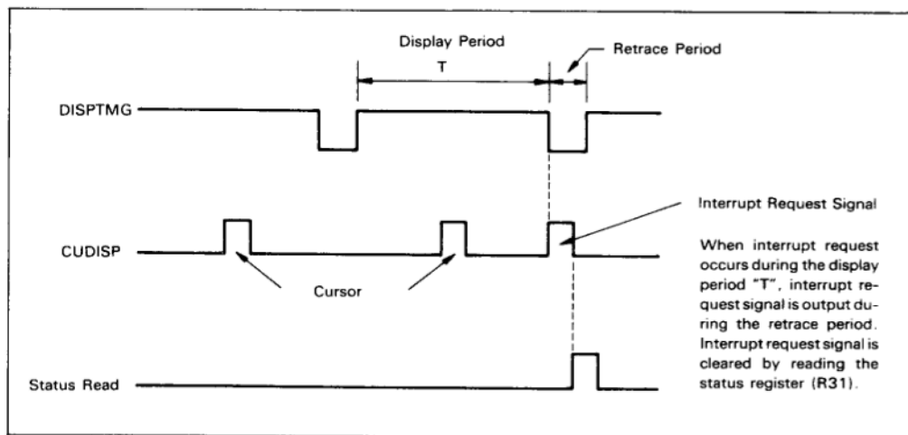
Figure 21 Interrupt Timing
