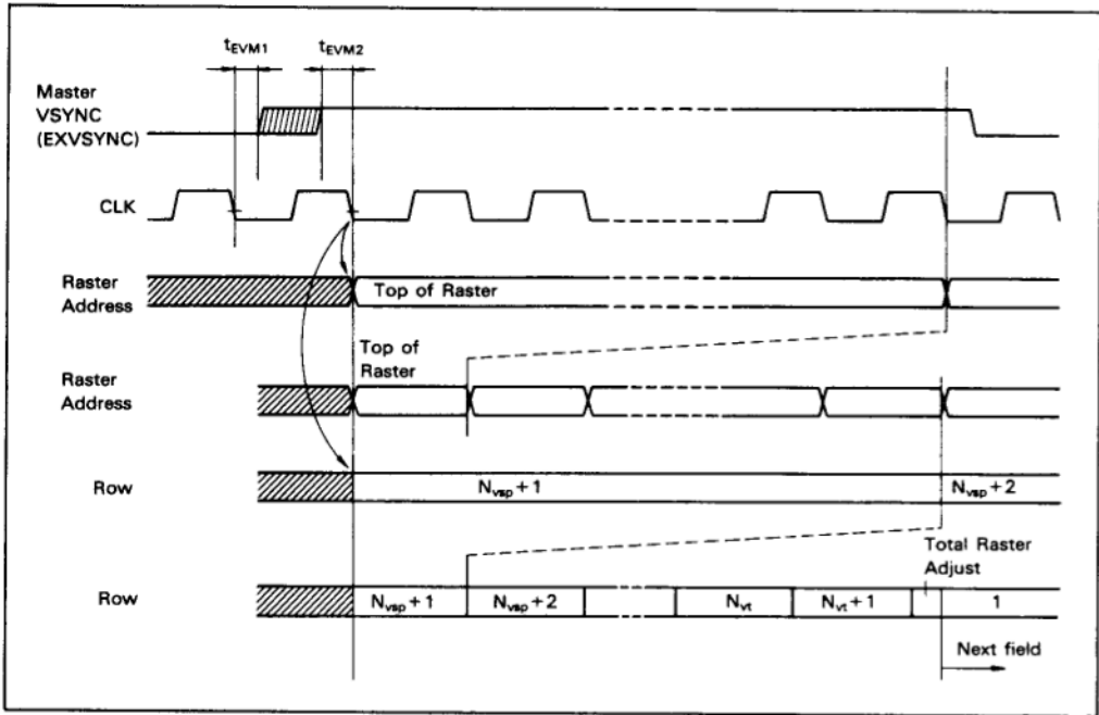
Figure 18 Synchronization Sequence
