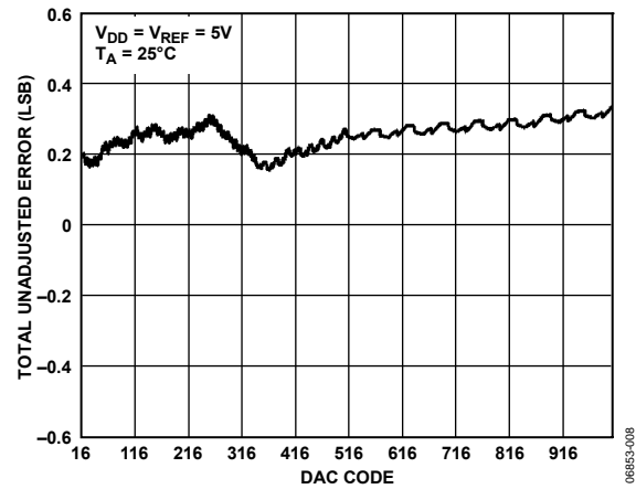
Figure 9. AD5611 Total Unadjusted Error (TUE)
