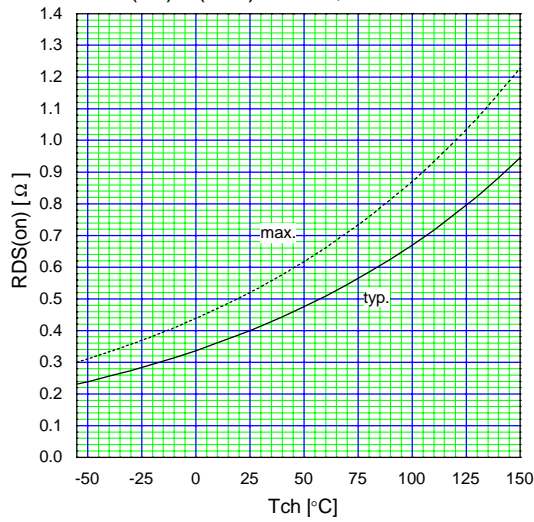
Drain-Source On-state Resistance R_{DS(on)}=f(T_{ch}):I_D=6A, V_{GS}=10V
