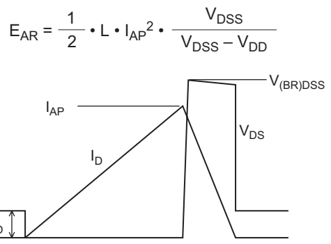
Avalanche Waveform
