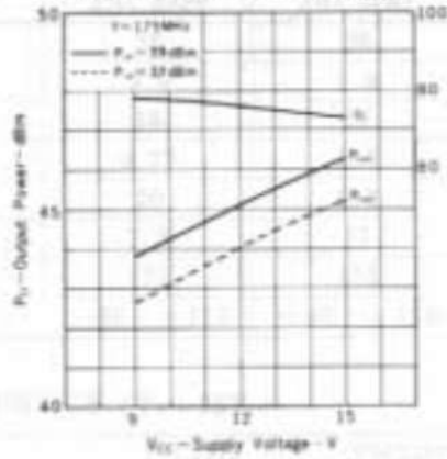
OUTPUT POWER & COLLECTOR EFFICIENCY vs. SUPPLY VOLTAGE
